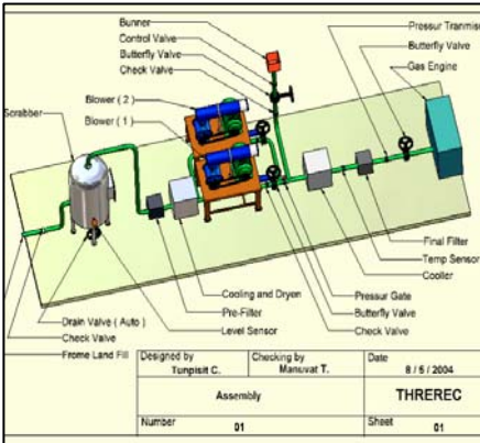
Process Diagram
